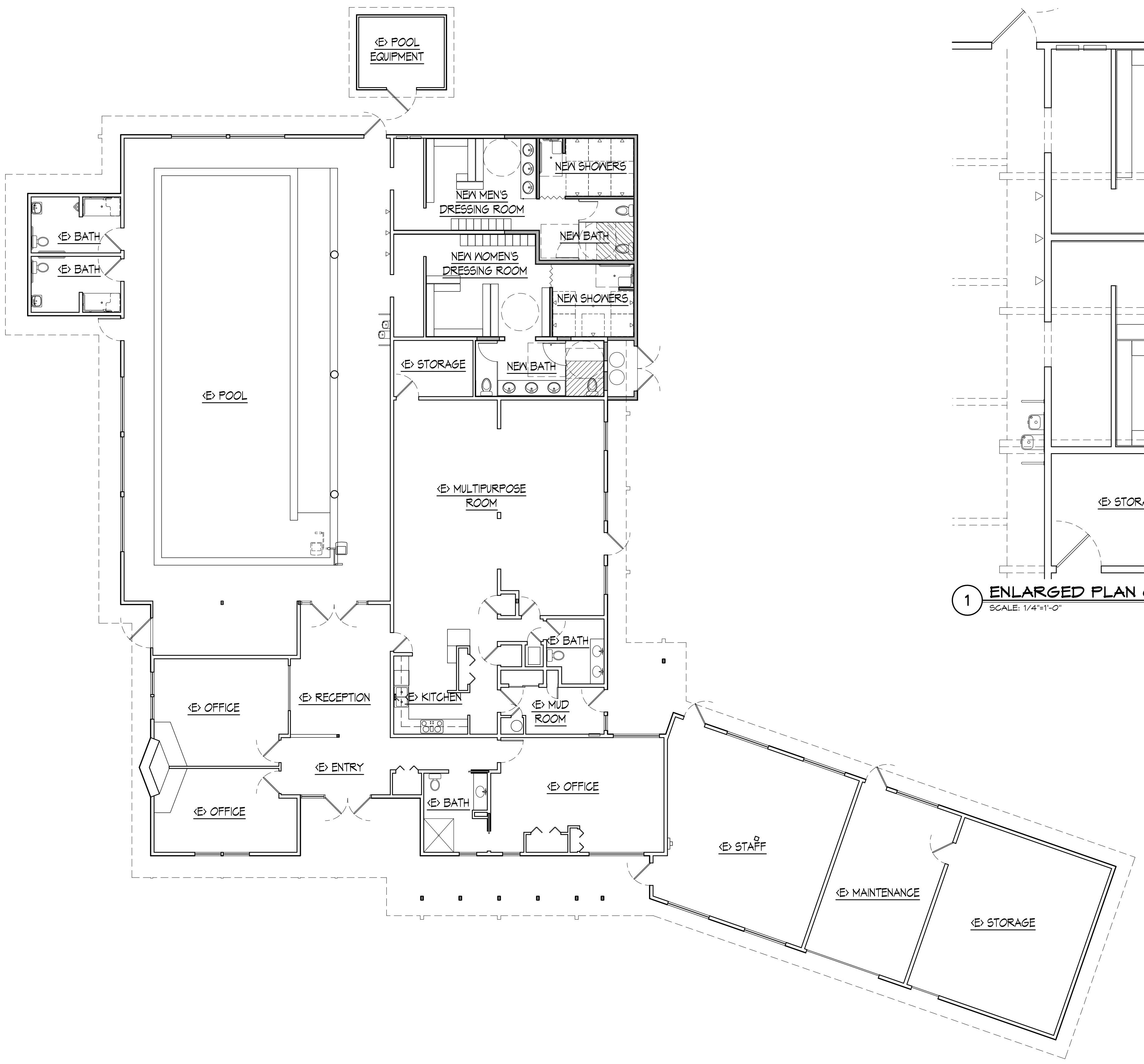
2 OVERALL FLOOR PLAN SCALE: 1/8"=1'-0"
