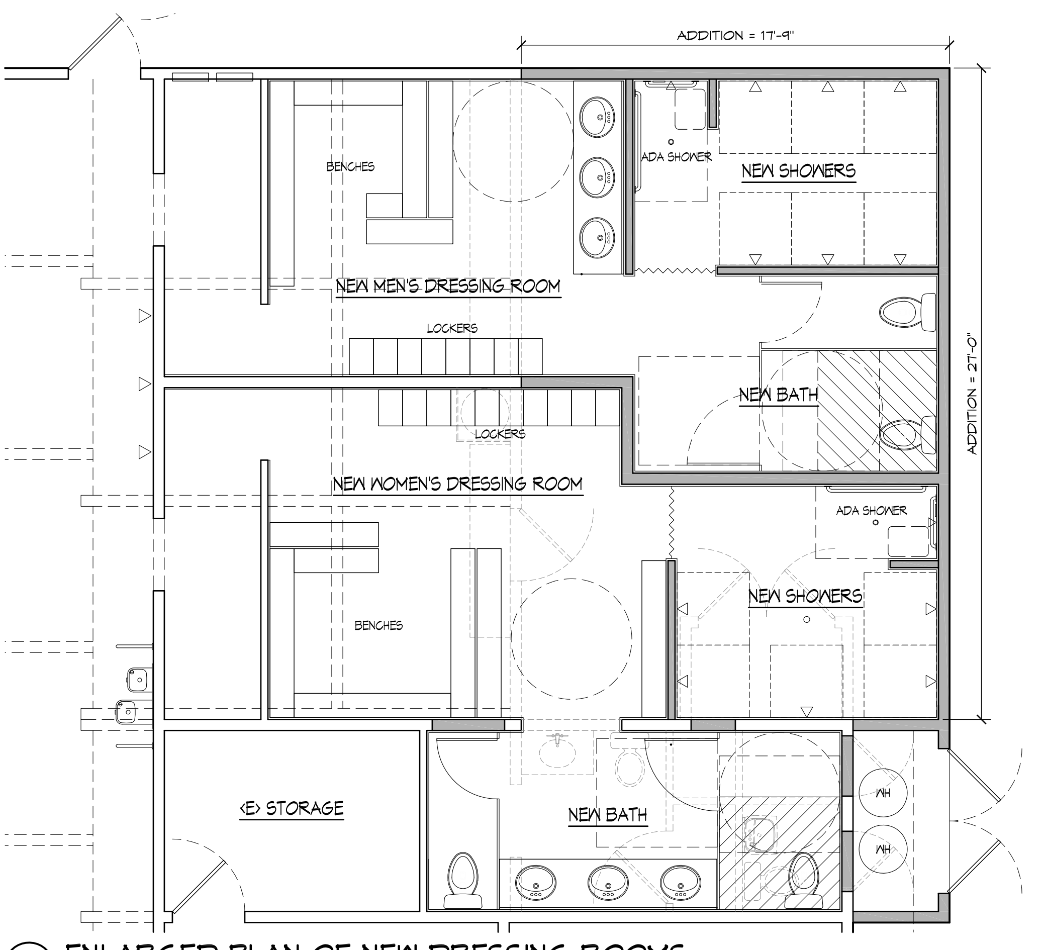
1 ENLARGED PLAN OF NEW DRESSING ROOMS SCALE: 1/4"=1'-0"
